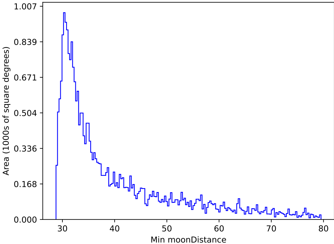
ddf_loaded_half_fl8_v3.4_10yrs All sky r band: Min moonDistance
