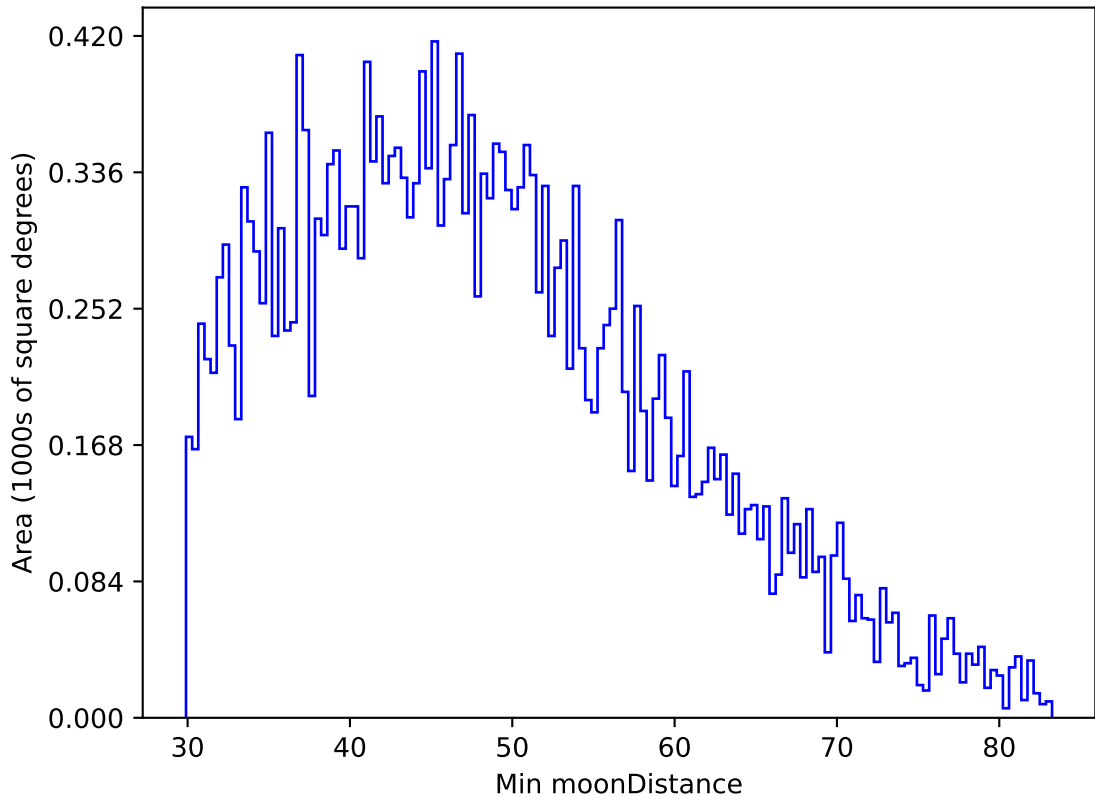
ddf_loaded_half_fl8_v3.4_10yrs All sky g band: Min moonDistance
