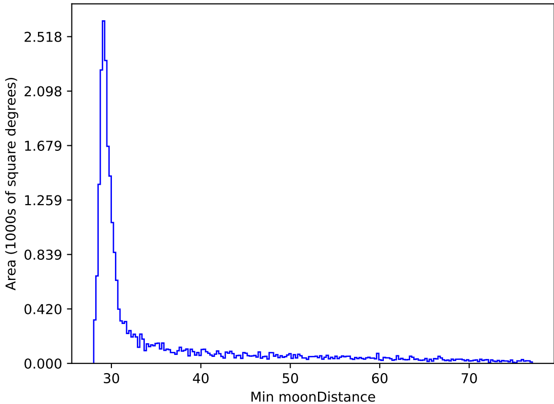
ddf_loaded_half_fl8_v3.4_10yrs All sky all bands: Min moonDistance
