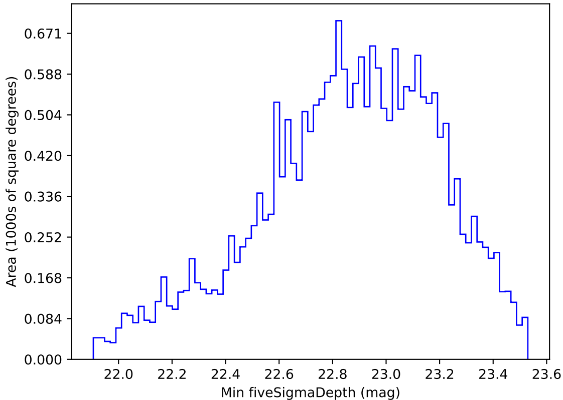
ddf_loaded_half_fl8_v3.4_10yrs Yr 1 u band: Min fiveSigmaDepth
