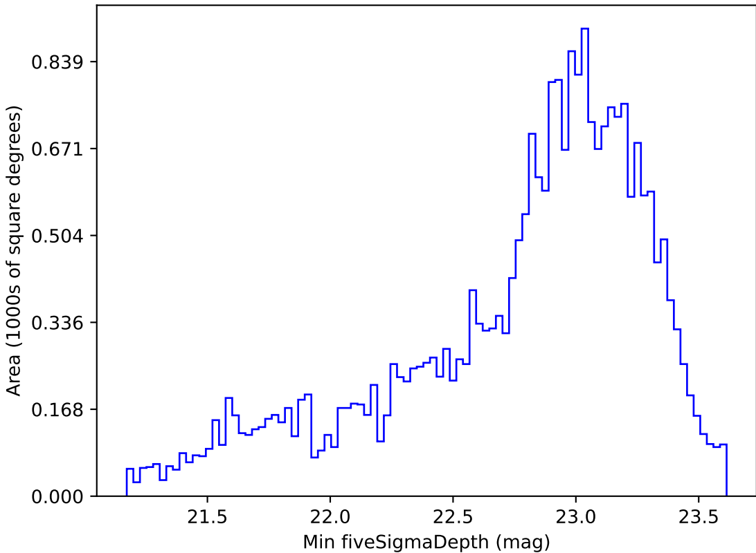
ddf_loaded_half_fl8_v3.4_10yrs Yr 1 i band: Min fiveSigmaDepth
