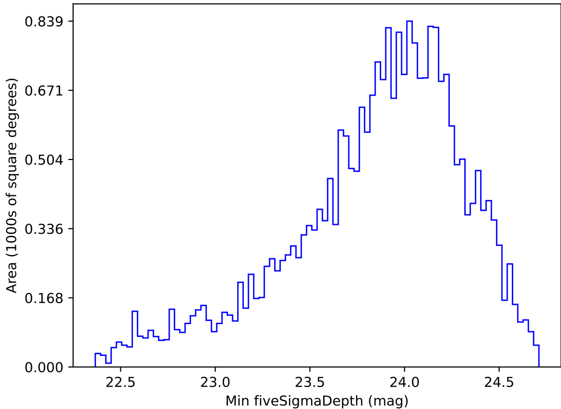
ddf_loaded_half_fl8_v3.4_10yrs Yr 1 g band: Min fiveSigmaDepth
