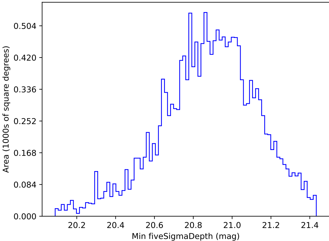
ddf_loaded_half_fl8_v3.4_10yrs WFD y band: Min fiveSigmaDepth
