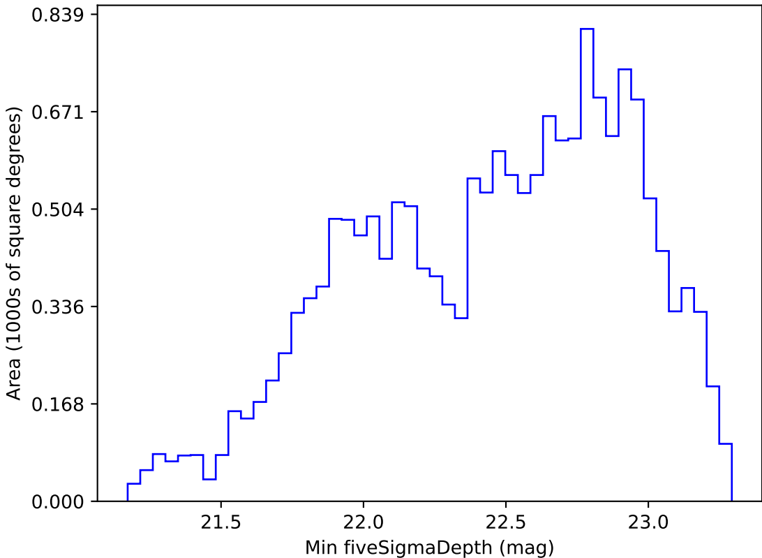
ddf_loaded_half_fl8_v3.4_10yrs WFD r band: Min fiveSigmaDepth
