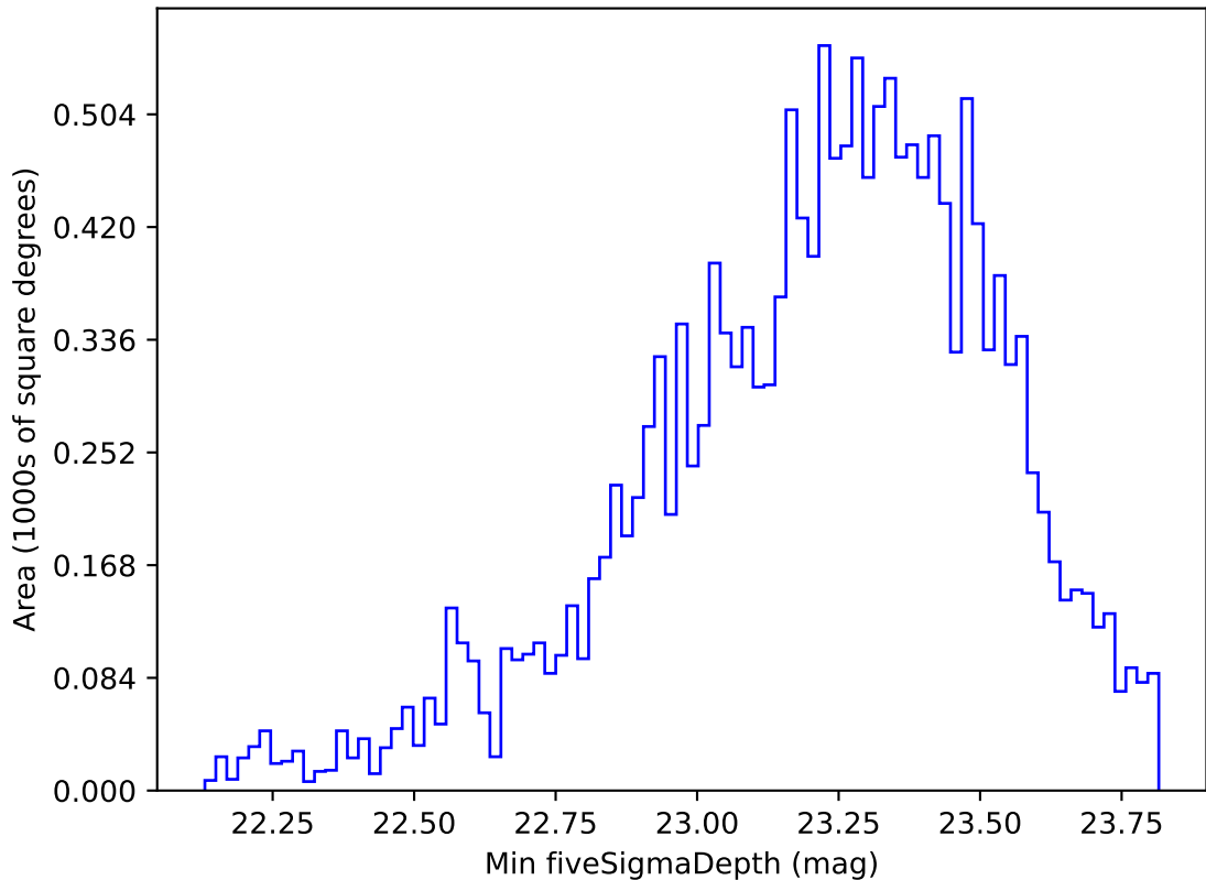
ddf_loaded_half_fl8_v3.4_10yrs WFD g band: Min fiveSigmaDepth
