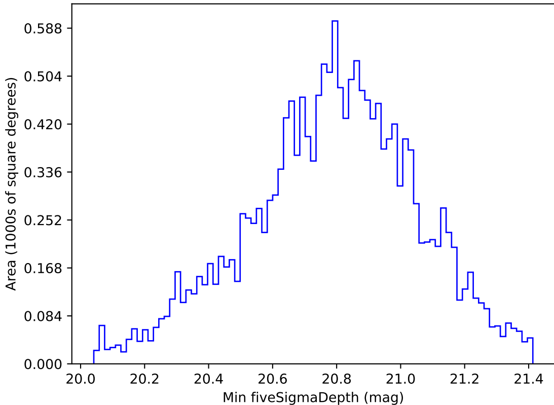
ddf_loaded_half_fl8_v3.4_10yrs WFD all bands: Min fiveSigmaDepth
