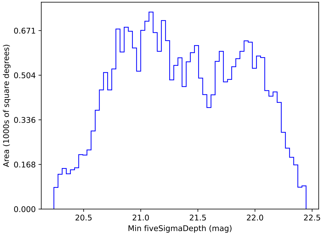
ddf_loaded_half_fl8_v3.4_10yrs All sky z band: Min fiveSigmaDepth
