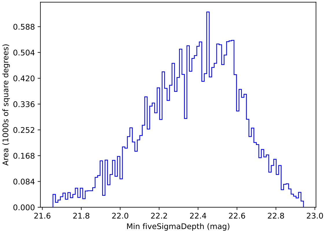
ddf_loaded_half_fl8_v3.4_10yrs All sky u band: Min fiveSigmaDepth
