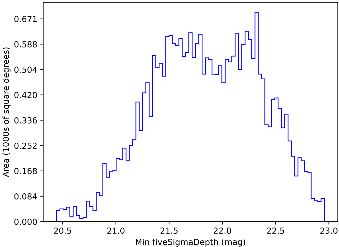
ddf_loaded_half_fl8_v3.4_10yrs All sky i band: Min fiveSigmaDepth
