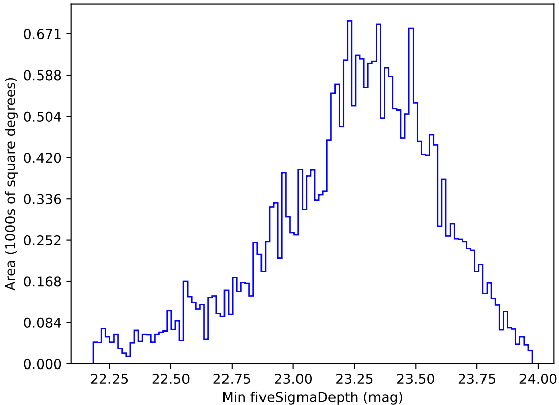
ddf_loaded_half_fl8_v3.4_10yrs All sky g band: Min fiveSigmaDepth
