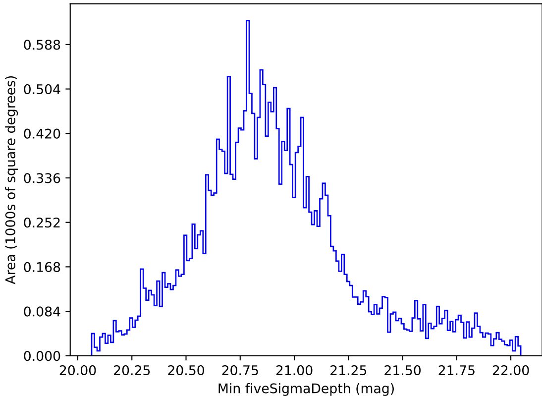
ddf_loaded_half_fl8_v3.4_10yrs All sky all bands: Min fiveSigmaDepth
