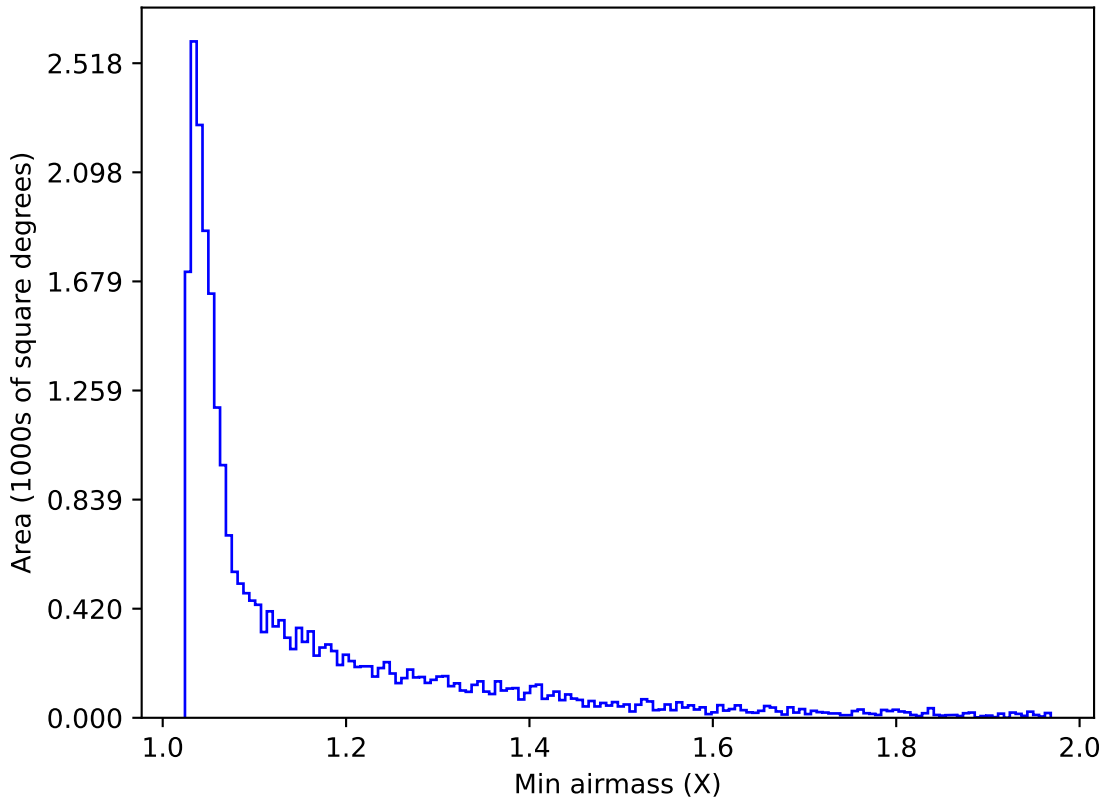
ddf_loaded_half_fl8_v3.4_10yrs Yr 1 r band: Min airmass
