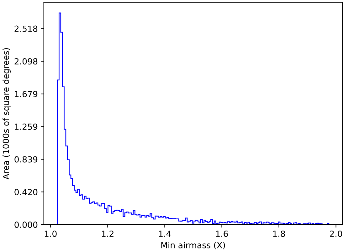
ddf_loaded_half_fl8_v3.4_10yrs Yr 1 i band: Min airmass
