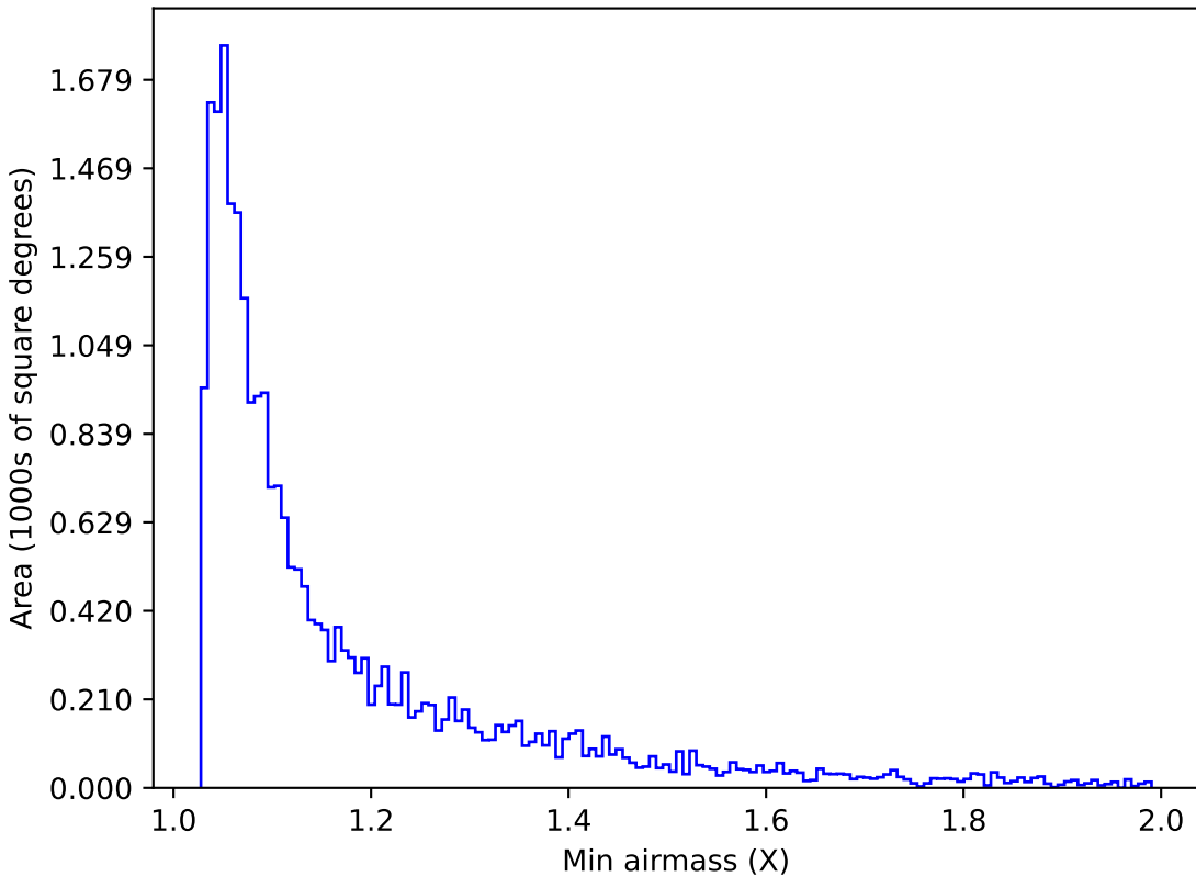
ddf_loaded_half_fl8_v3.4_10yrs Yr 1 g band: Min airmass
