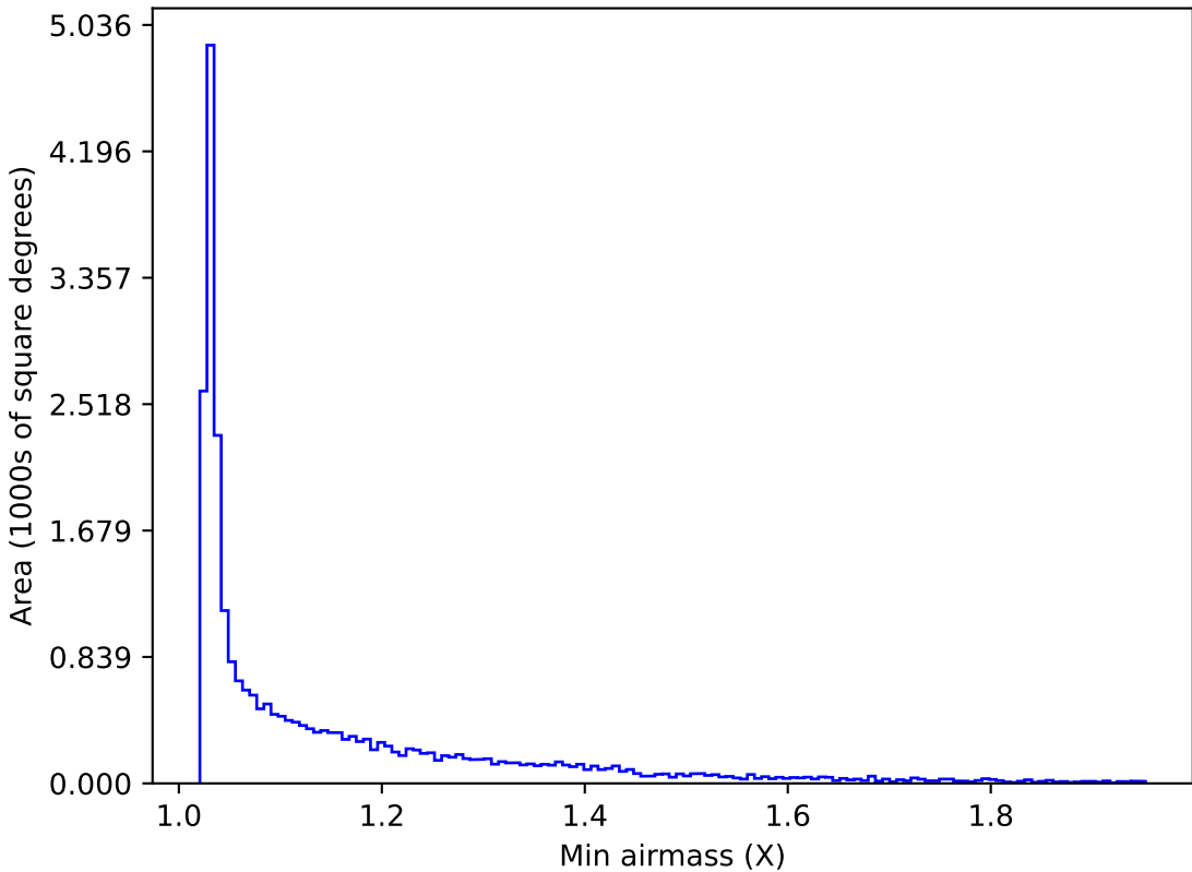
ddf_loaded_half_fl8_v3.4_10yrs Yr 1 all bands: Min airmass
