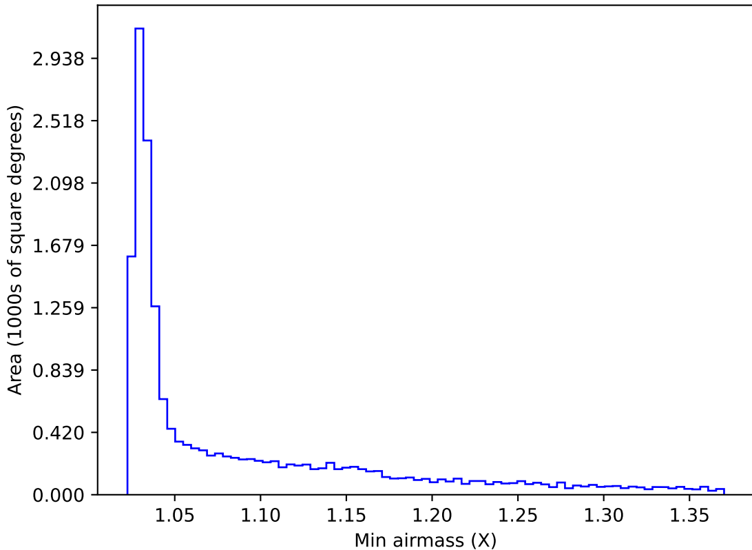
ddf_loaded_half_f18_v3.4_10yrs WFD y band: Min airmass
