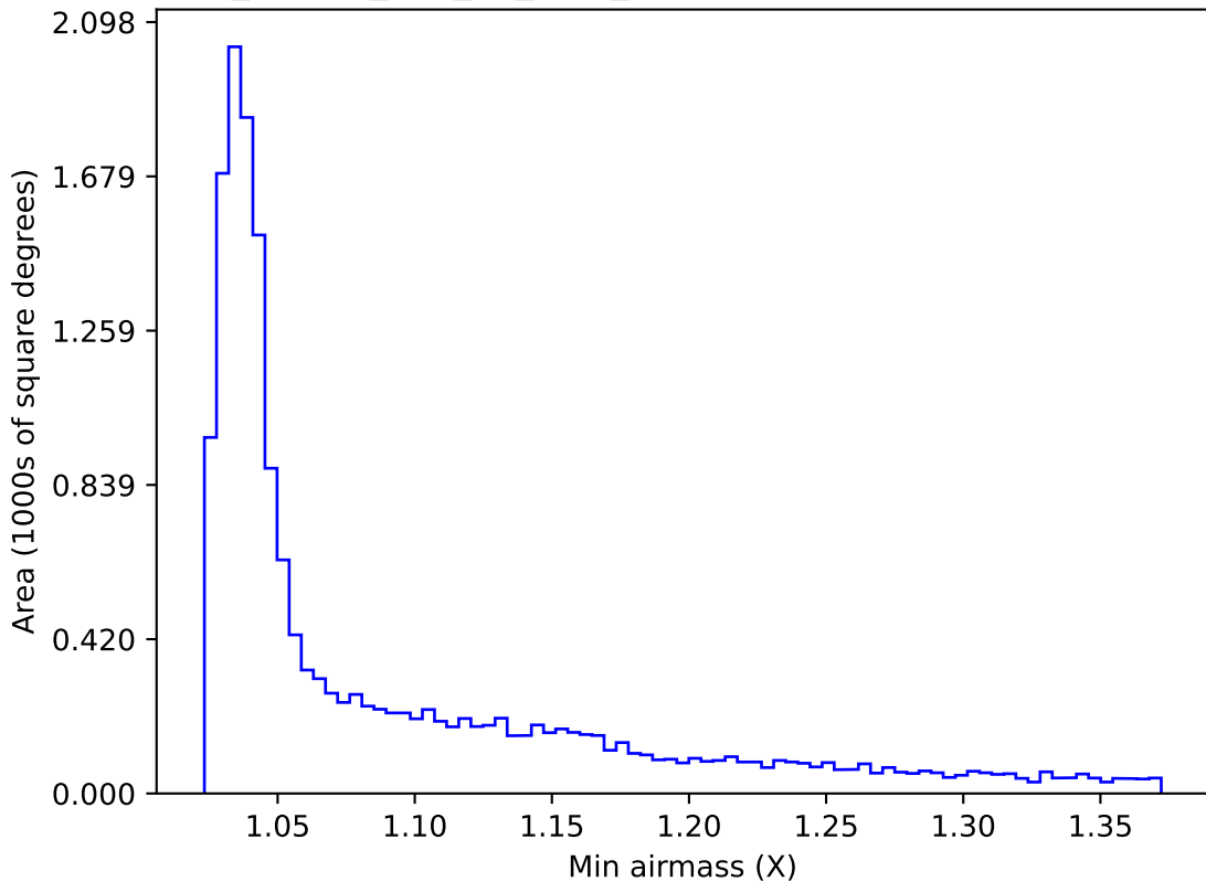
ddf_loaded_half_f18_v3.4_10yrs WFD g band: Min airmass
