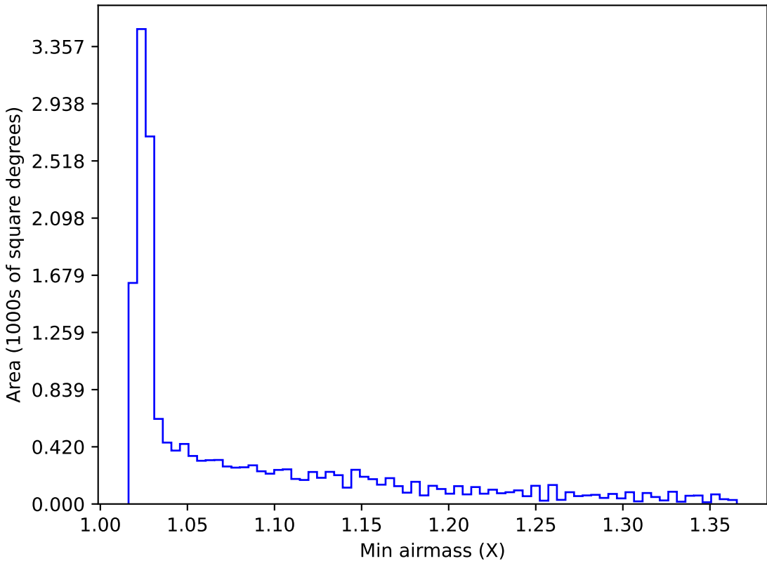
ddf_loaded_half_fl8_v3.4_10yrs WFD all bands: Min airmass
