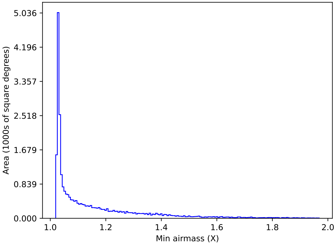
ddf_loaded_half_fl8_v3.4_10yrs All sky z band: Min airmass
