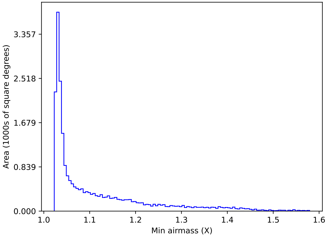
ddf_loaded_half_fl8_v3.4_10yrs All sky y band: Min airmass
