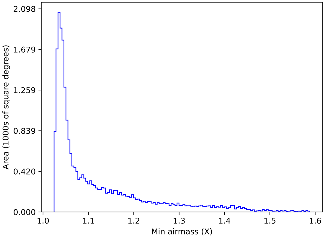
ddf_loaded_half_fl8_v3.4_10yrs All sky u band: Min airmass
