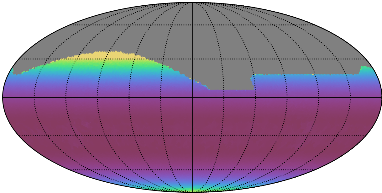
ddf_loaded_half_fl8_v3.4_10yrs All sky r band: Min airmass
