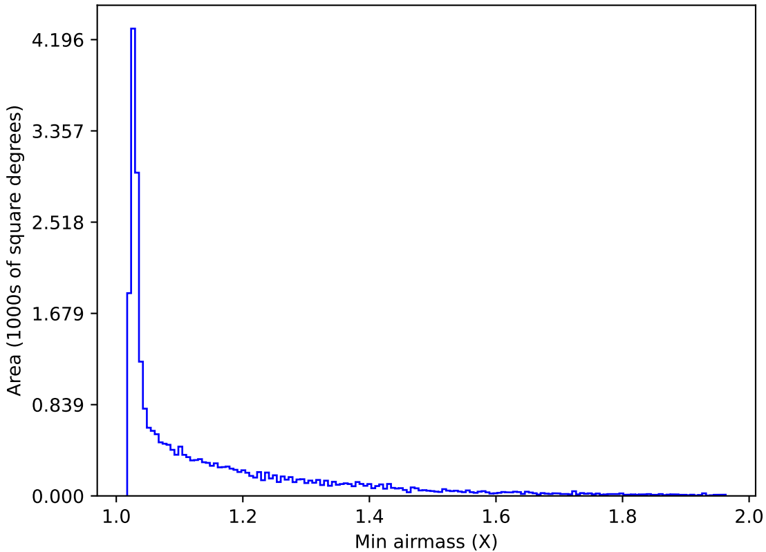
ddf_loaded_half_fl8_v3.4_10yrs All sky r band: Min airmass
