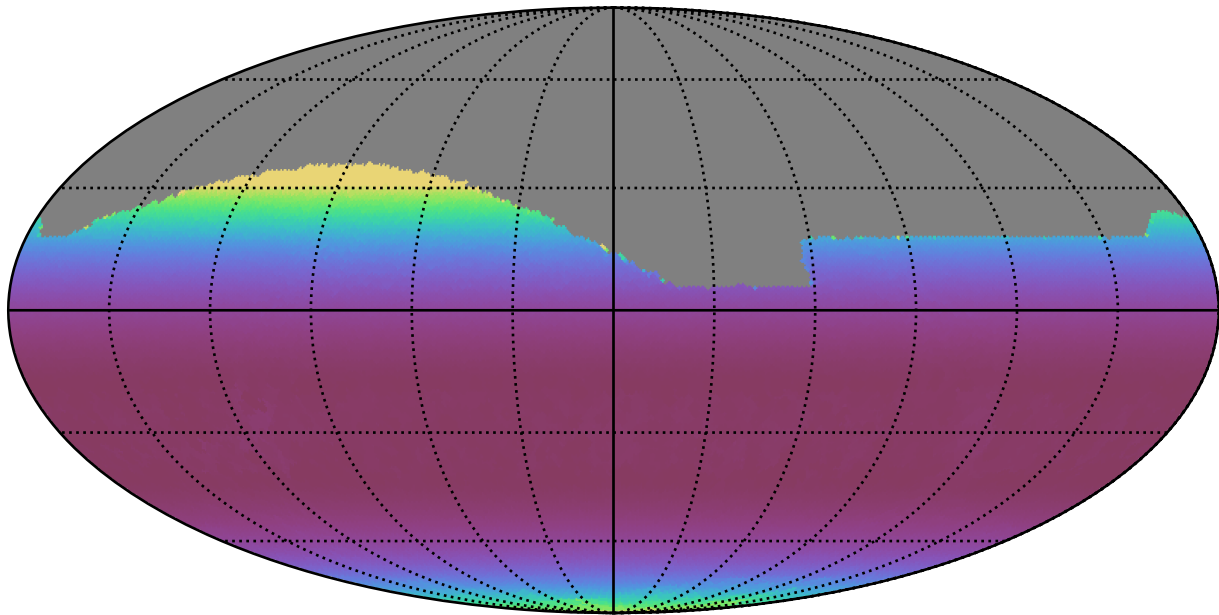
ddf_loaded_half_fl8_v3.4_10yrs All sky i band: Min airmass
