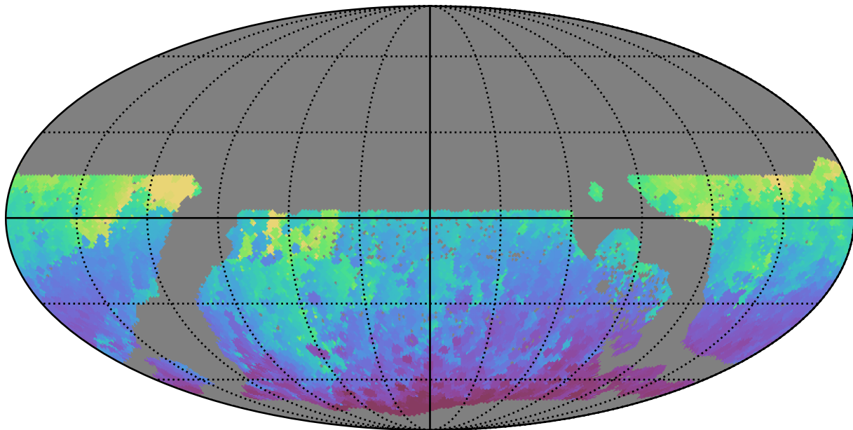
ddf_loaded_half_fl8_v3.4_10yrs WFD z band: Min HA
