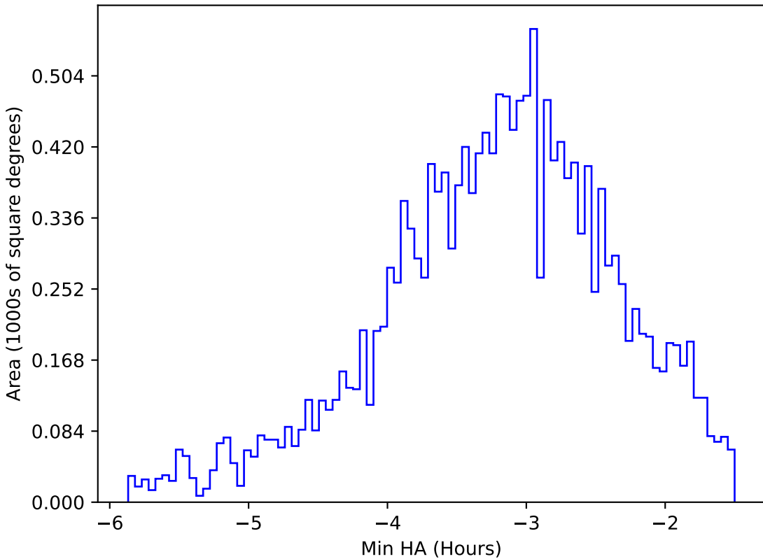
ddf_loaded_half_fl8_v3.4_10yrs WFD u band: Min HA
