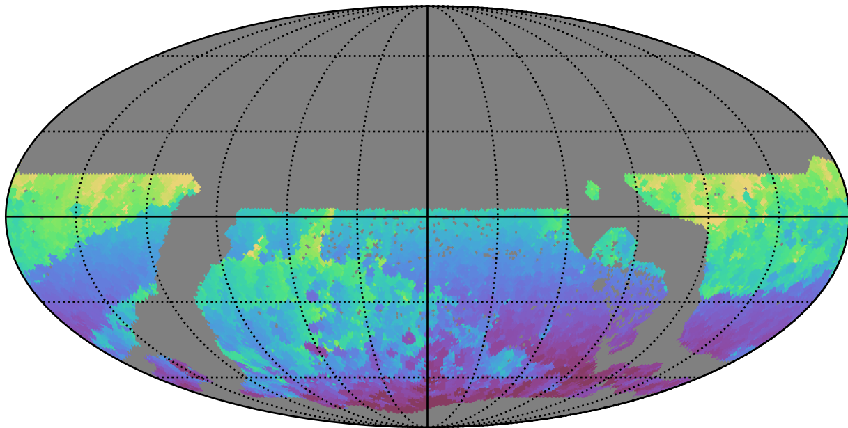
ddf_loaded_half_fl8_v3.4_10yrs WFD r band: Min HA
