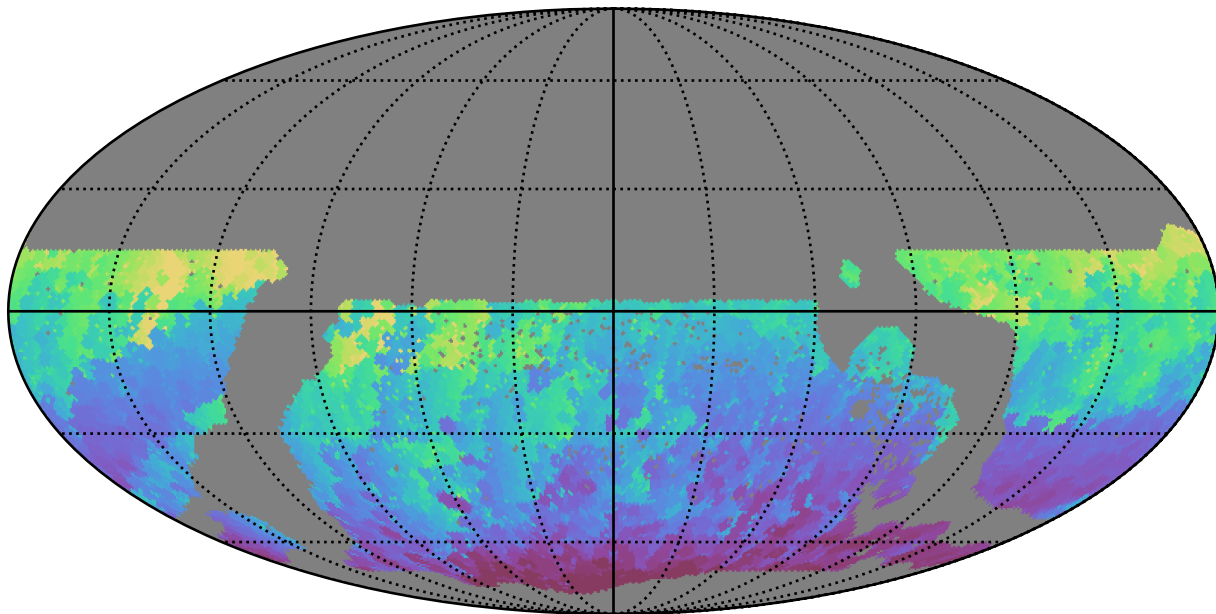
ddf_loaded_half_fl8_v3.4_10yrs WFD i band: Min HA
