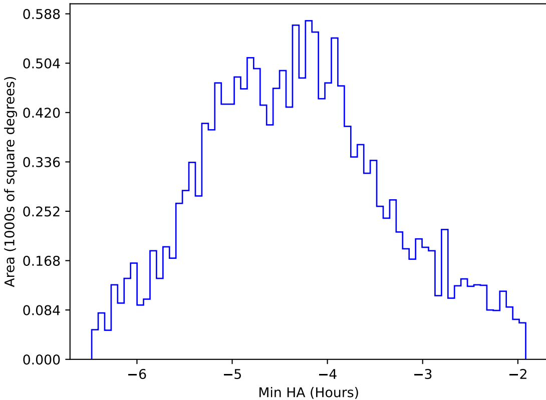
ddf_loaded_half_fl8_v3.4_10yrs WFD i band: Min HA
