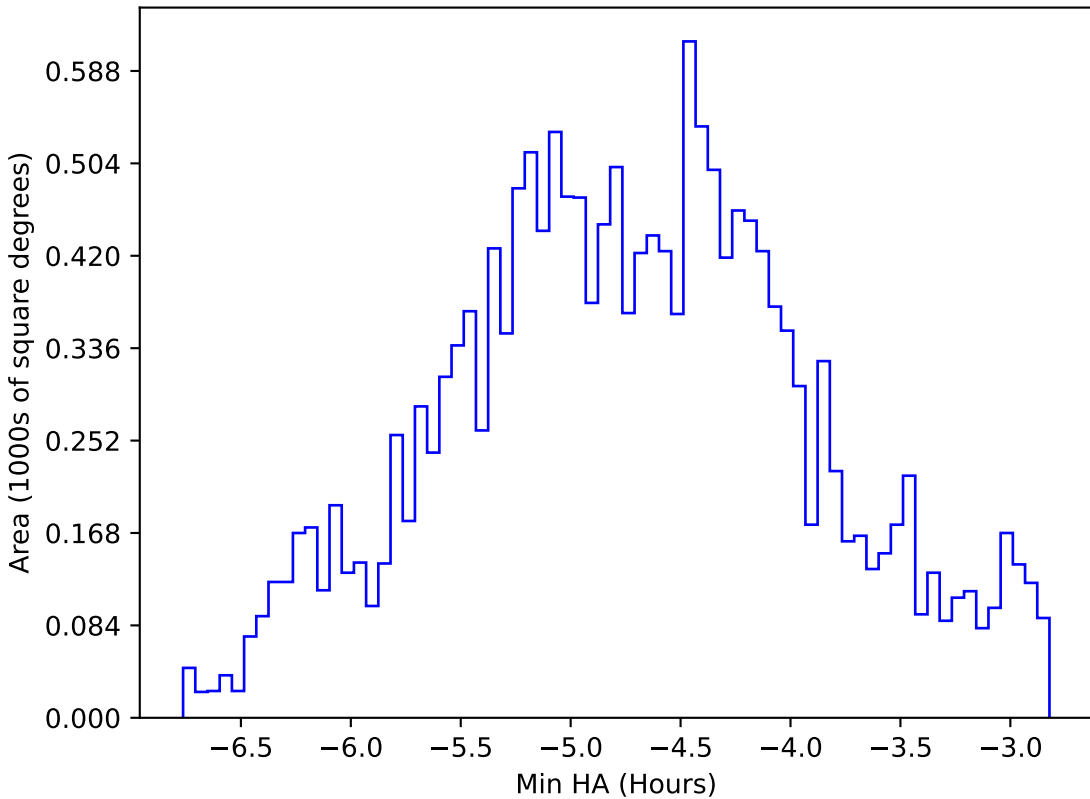
ddf_loaded_half_fl8_v3.4_10yrs WFD all bands: Min HA
