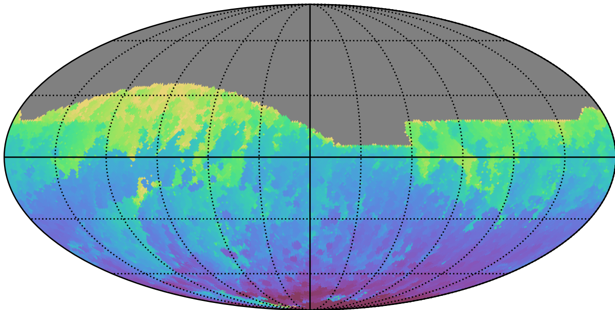
ddf_loaded_half_fl8_v3.4_10yrs All sky z band: Min HA
