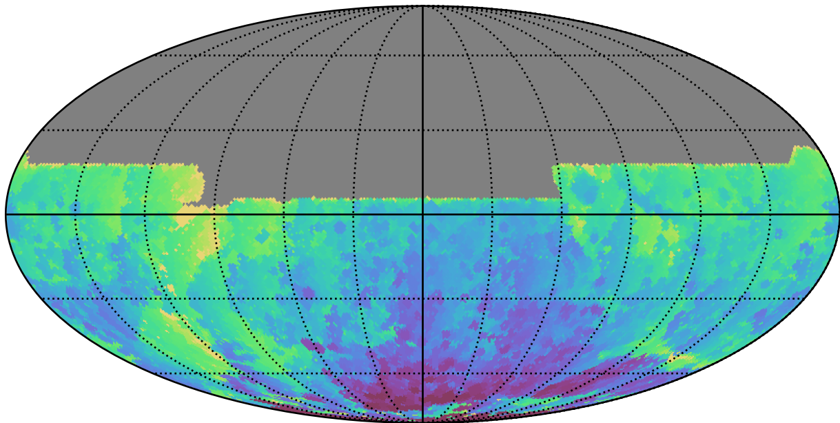
ddf_loaded_half_fl8_v3.4_10yrs All sky y band: Min HA
