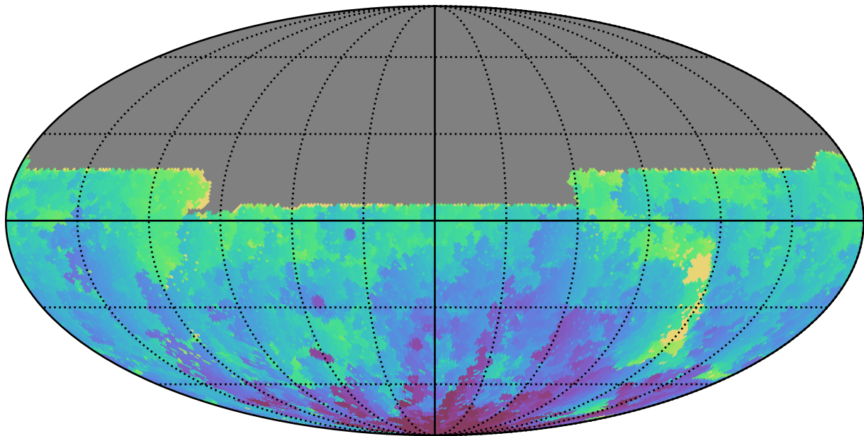
ddf_loaded_half_f18_v3.4_10yrs All sky u band: Min HA
