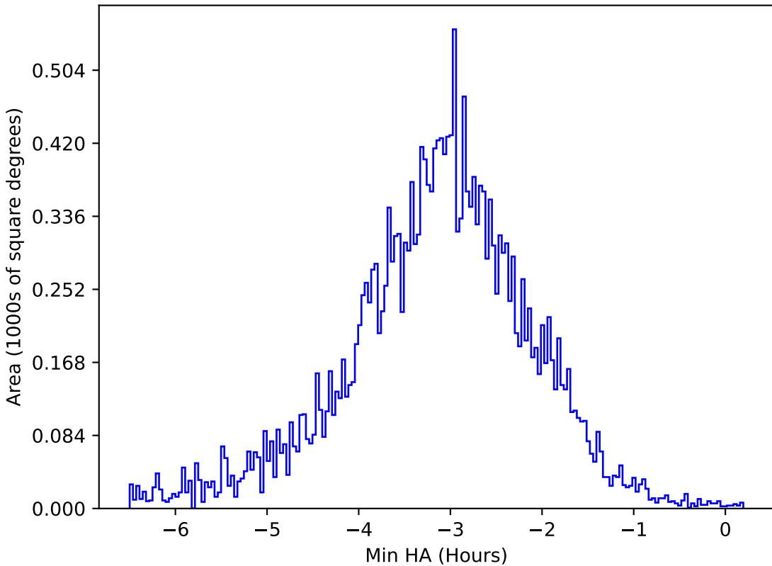
ddf_loaded_half_f18_v3.4_10yrs All sky u band: Min HA
