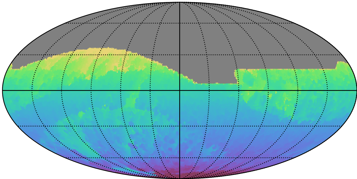
ddf_loaded_half_fl8_v3.4_10yrs All sky all bands: Min HA
