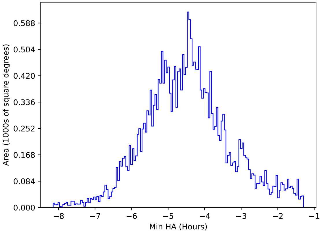
ddf_loaded_half_fl8_v3.4_10yrs All sky all bands: Min HA
