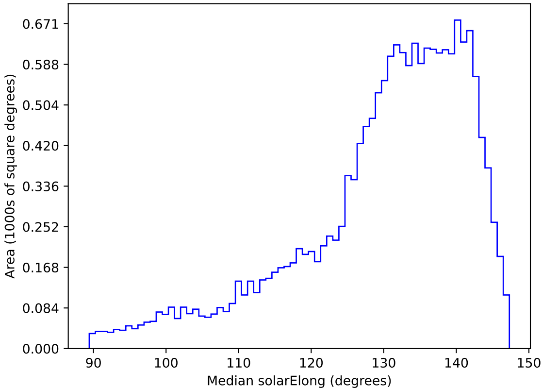
ddf_loaded_half_fl8_v3.4_10yrs WFD y band: Median solarElong
