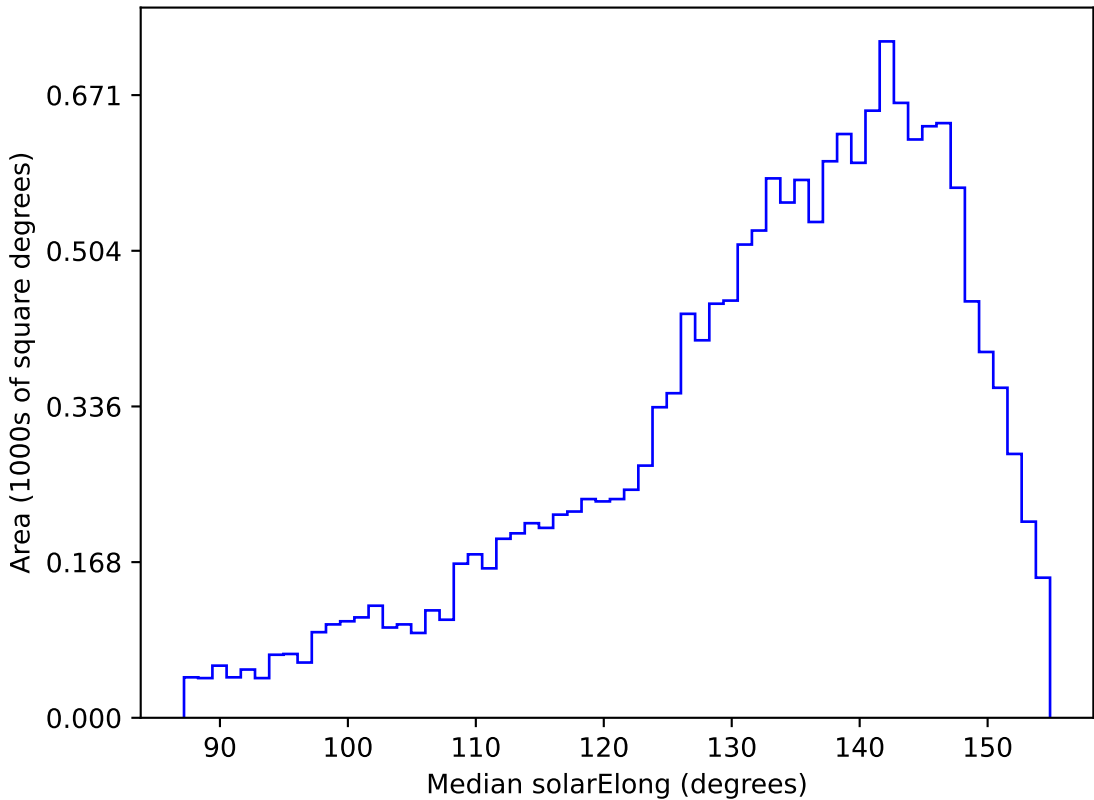
ddf_loaded_half_fl8_v3.4_10yrs WFD u band: Median solarElong
