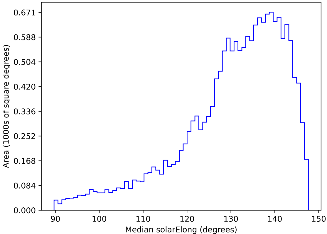
ddf_loaded_half_fl8_v3.4_10yrs WFD r band: Median solarElong
