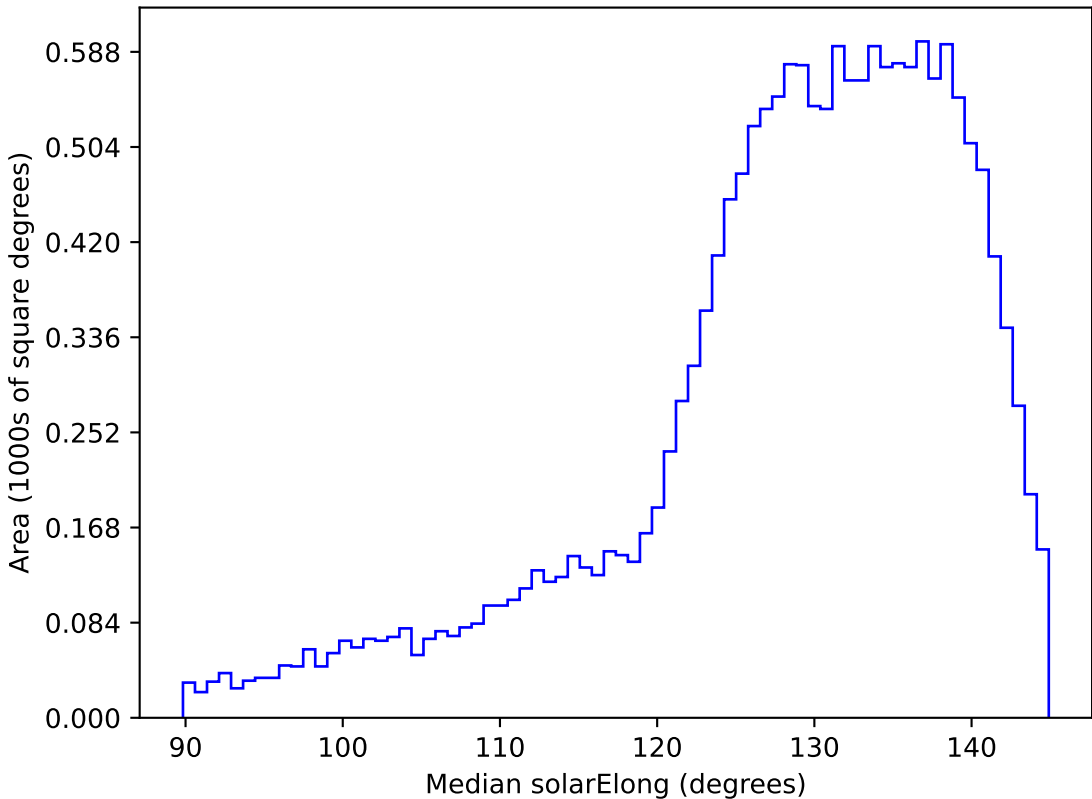
ddf_loaded_half_fl8_v3.4_10yrs WFD i band: Median solarElong
