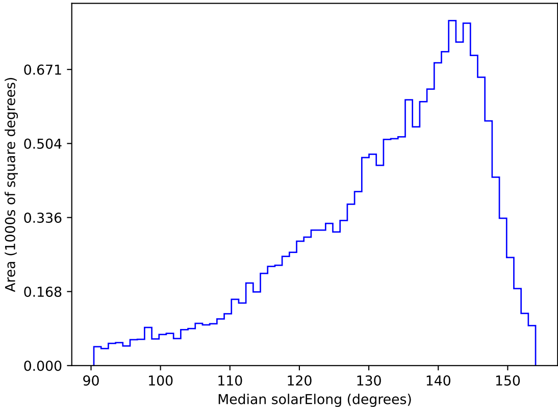
ddf_loaded_half_fl8_v3.4_10yrs WFD g band: Median solarElong
