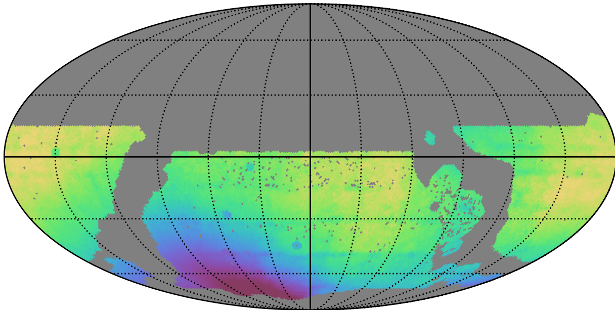
ddf_loaded_half_fl8_v3.4_10yrs WFD all bands: Median solarElong
