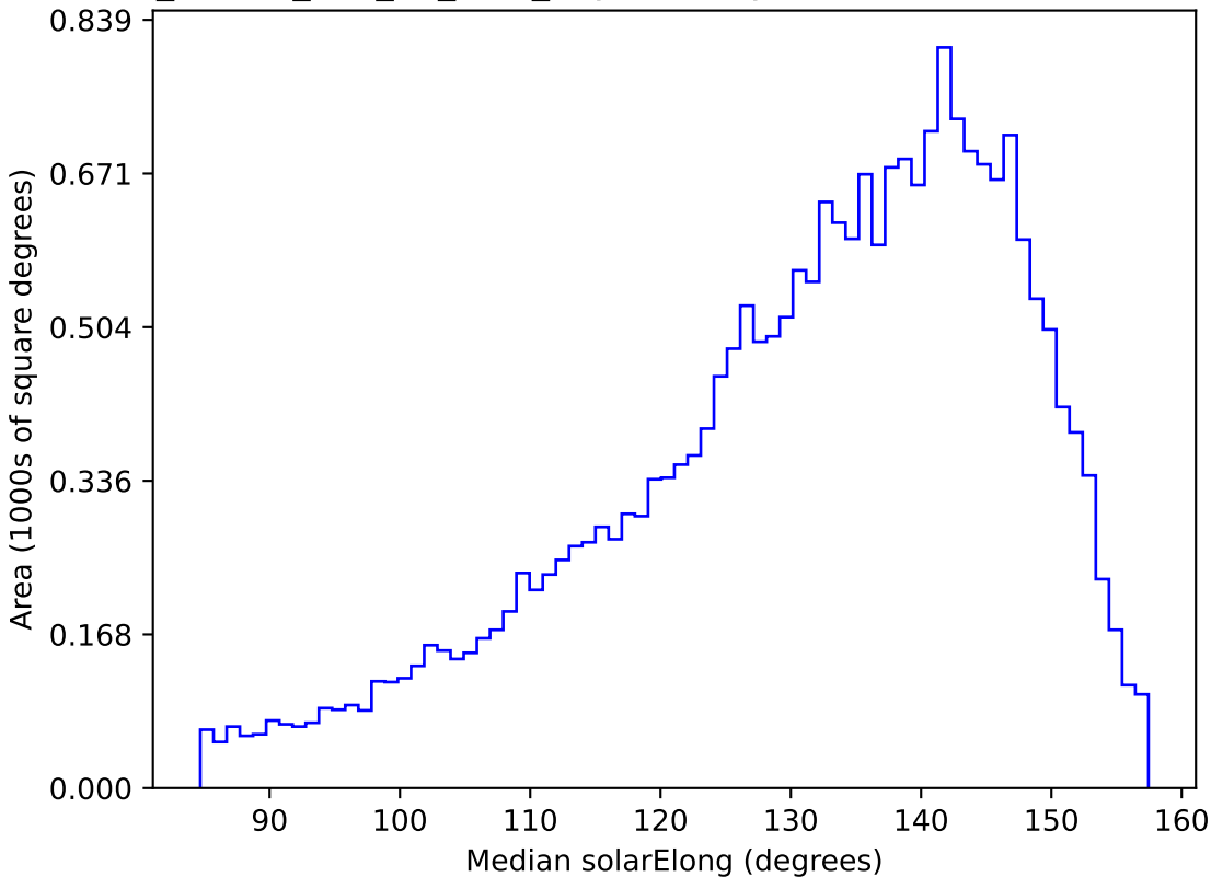
ddf_loaded_half_fl8_v3.4_10yrs All sky u band: Median solarElong
