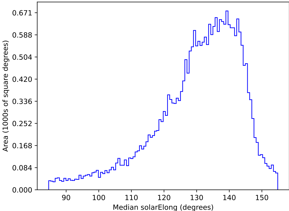
ddf_loaded_half_fl8_v3.4_10yrs All sky r band: Median solarElong
