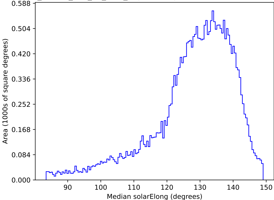
ddf_loaded_half_fl8_v3.4_10yrs All sky i band: Median solarElong
