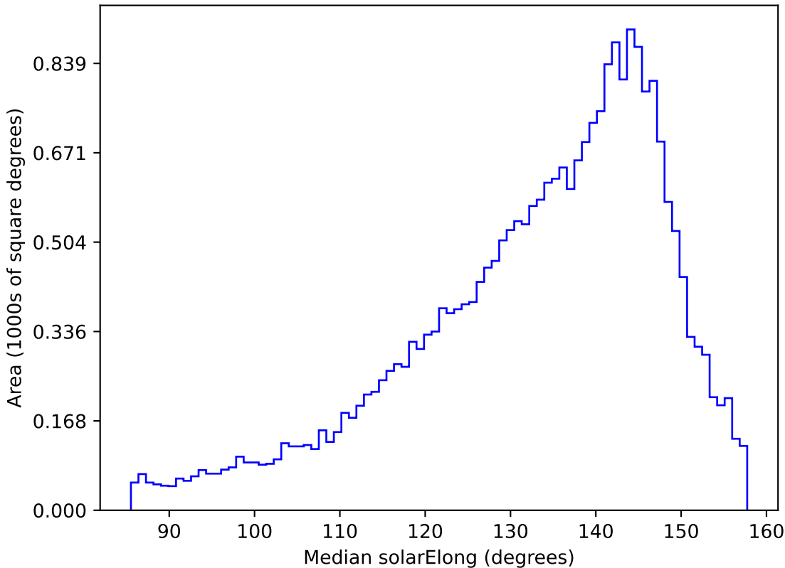
ddf_loaded_half_fl8_v3.4_10yrs All sky g band: Median solarElong
